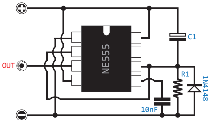
DELAY ON
