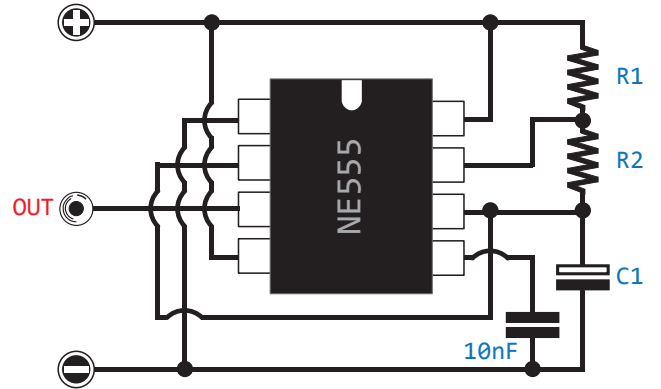
ASTABLE
