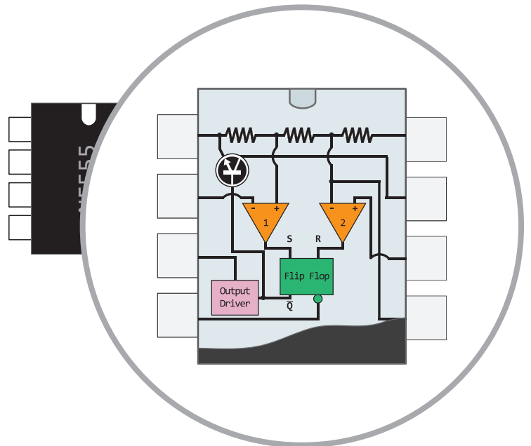
ASTABLE
