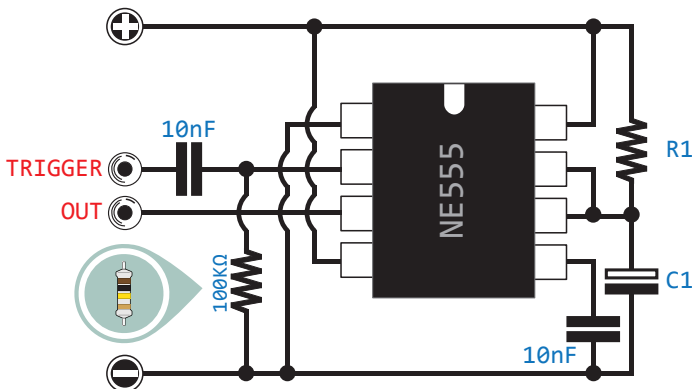
MONOSTABLE
