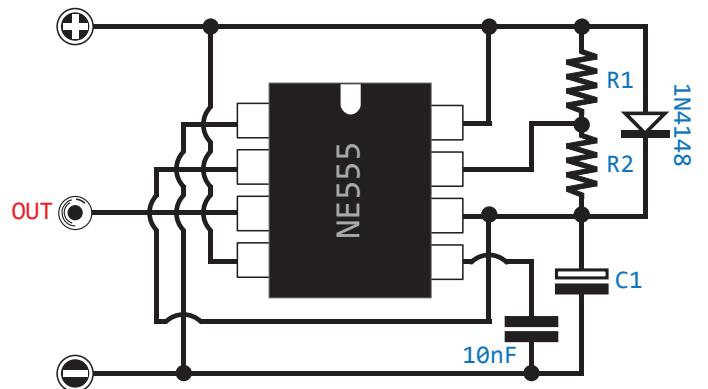
ASTABLE
