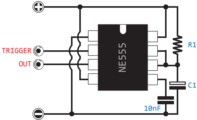
MONOSTABLE
